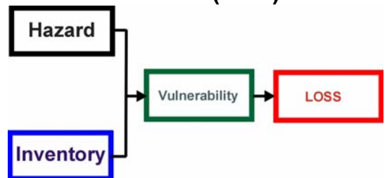
Structure of a Catastrophe (CAT) Model
