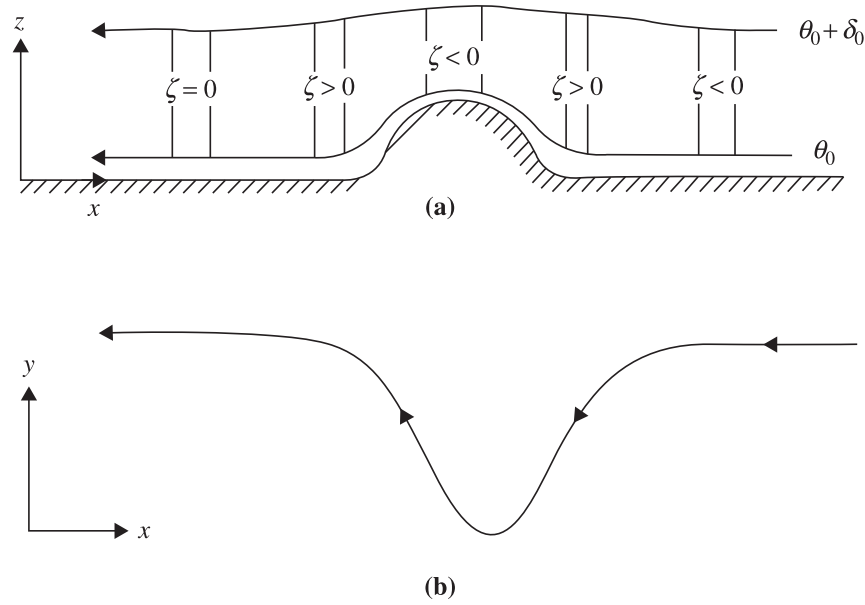
FIGURE 4.12 As in Figure 4.11, but for easterly flow.
