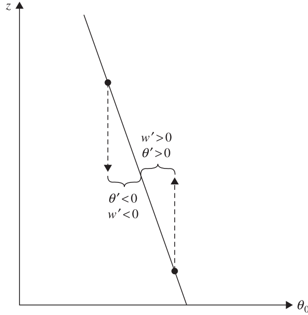
FIGURE 8.1 Correlation between vertical velocity and potential temperature perturbations for upward or downward parcel displacements when the mean potential temperature \theta_0(z) decreases with height.
