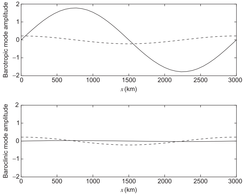
FIGURE 7.12 Zonal distribution of the amplitude of a transient neutral disturbance initially confined entirely to the upper layer in the two-layer model. Dashed lines show the initial distribution of the baroclinic and barotropic modes; solid lines show the distribution at the time of maximum amplification.
