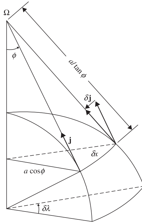
FIGURE 2.3 Dependence of unit vector \mathbf{j} on longitude.
