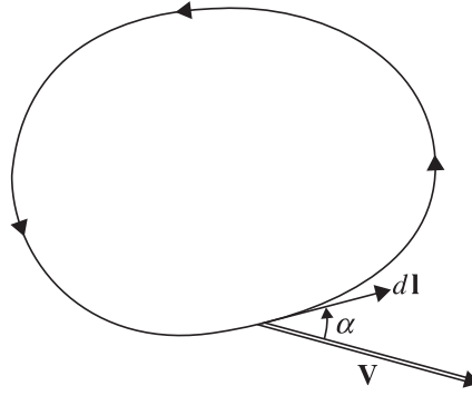
FIGURE 4.1 Circulation about a closed contour.
