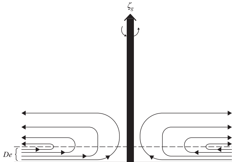
FIGURE 8.8 Streamlines of the secondary circulation forced by frictional convergence in the planetary boundary layer for a cyclonic vortex in a stably stratified baroclinic atmosphere. The circulation decays with height in the interior.
