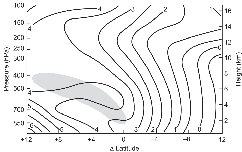
FIGURE 11.8 Absolute vorticity (units 10^{-5}\text{s}^{-1} ) corresponding to the mean wind field of Figure 11.6. Shading shows region where \beta - \partial^2 \bar{u} / \partial y^2 is negative. (After Reed et al., 1977. Copyright © American Meteorological Society. Reprinted with permission.)
