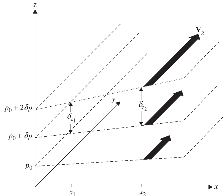
FIGURE 3.8 Relationship between vertical shear of the geostrophic wind and horizontal thickness gradients. (Note that \delta p < 0 .)
