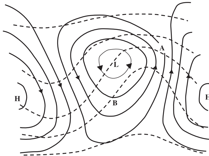
FIGURE 9.2 Schematic surface isobars ( solid lines ) and isotherms ( dashed lines ) for a baroclinic wave disturbance. Arrows show direction of geostrophic wind. Horizontal stretching deformation intensifies the temperature gradient at A, and horizontal shear deformation intensifies the gradient at B. (After Hoskins and Bretherton, 1972. Copyright © American Meteorological Society. Reprinted with permission.)
