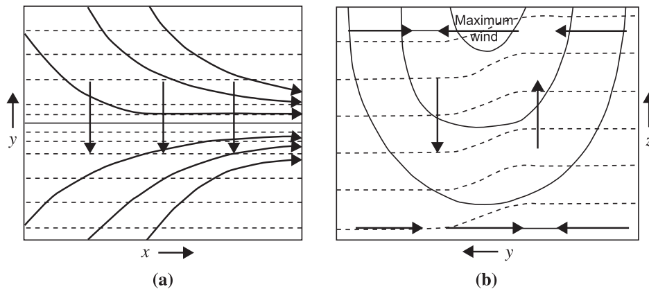
FIGURE 9.3 (a) Horizontal streamlines, isotherms, and \mathbf{Q} -vectors in a frontogenetic confluence. (b) Vertical section across the confluence showing isotachs ( solid lines ), isotherms ( dashed lines ), and vertical and transverse motions ( arrows ). (After Sawyer, 1956. Copyright © The Royal Society. Reprinted with permission.)
