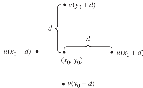
FIGURE 3.10 Grid for estimation of the horizontal divergence.
