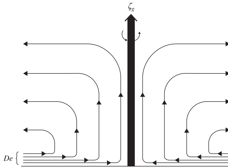
FIGURE 8.7 Streamlines of the secondary circulation forced by frictional convergence in the planetary boundary layer for a cyclonic vortex in a barotropic atmosphere. The circulation extends throughout the full depth of the vortex.
