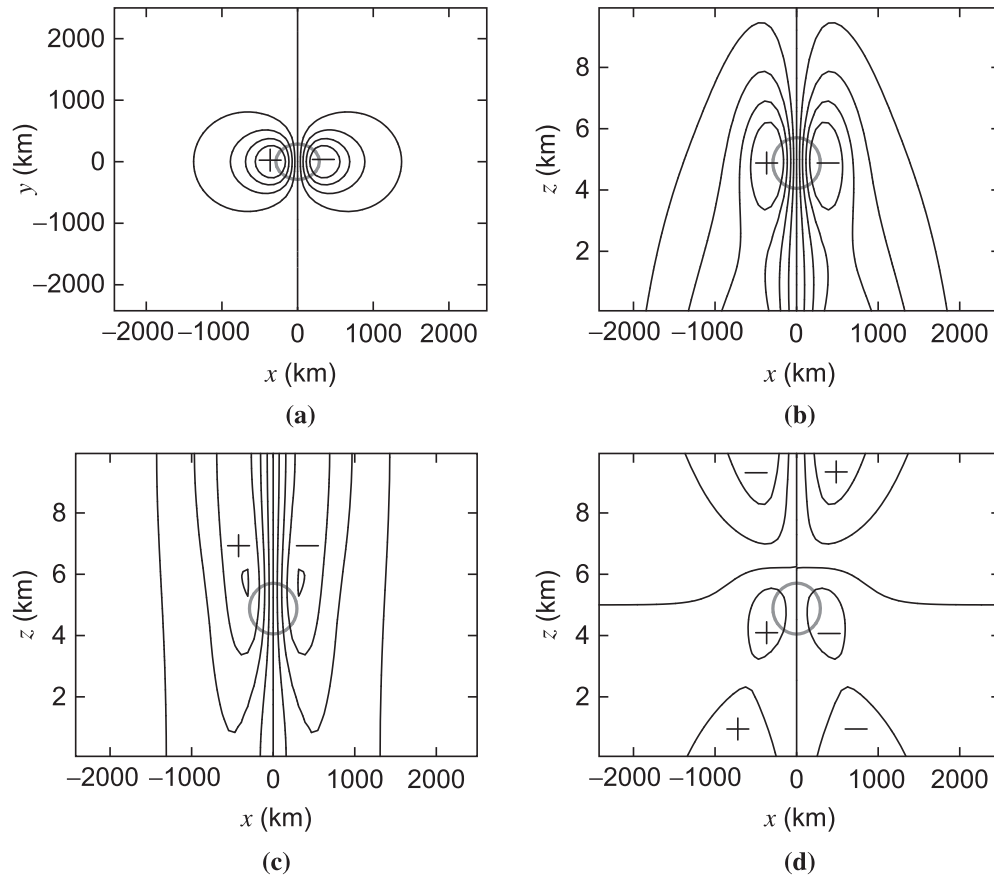
FIGURE 6.13 Pressure tendency associated with the PV blob in vertical shear shown in Figure 6.10. Pressure tendency: (a) plan view at 5-km altitude; (b) cross-section along y=0 ; (c) cross-section along y=0 of vorticity advection contribution; and (d) cross-section along y=0 of temperature advection contribution. The sum of (c) and (d) equals (b). Pressure tendency contours are shown every 5 hPa (\text{day})^{-1} , and the 1-PVU QG PV contour by a thick gray line.
