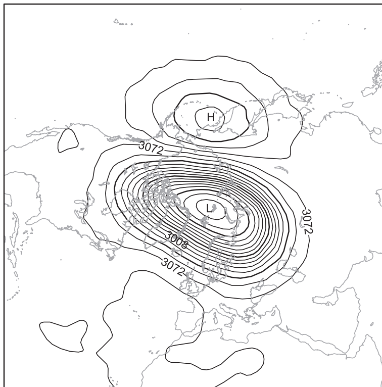
FIGURE 12.10 10-hPa geopotential height analyses for days in 1979: February 11 (a), February 16 (b), and February 21 (c) at 12 UTC, showing breakdown of the polar vortex associated with a wave number 2's sudden stratospheric warming. Contour interval: 16 dam. ( Analysis from ERA-40 reanalysis courtesy of the European Centre for Medium-Range Weather Forecasts. )
