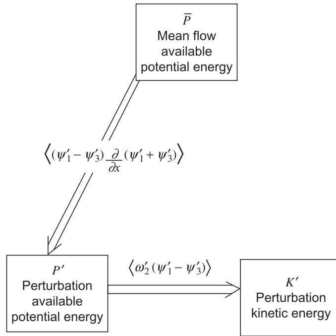
FIGURE 7.9 Energy flow in an amplifying baroclinic wave.
