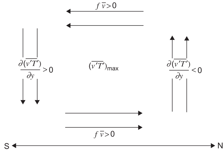
FIGURE 10.4 Schematic Eulerian mean meridional circulation forced by poleward heat fluxes.
