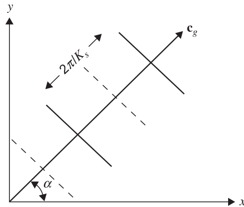
FIGURE 10.15 Stationary plane Rossby wave in a westerly flow. Ridges ( solid lines ) and troughs ( dashed lines ) are oriented at an angle \alpha to the y axis; the group velocity relative to the ground, c_g , is oriented at an angle \alpha to the x axis. The wavelength is 2\pi/K_s . (Adapted from Hoskins, 1983.)
