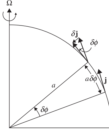
FIGURE 2.4 Dependence of unit vector \mathbf{j} on latitude.
