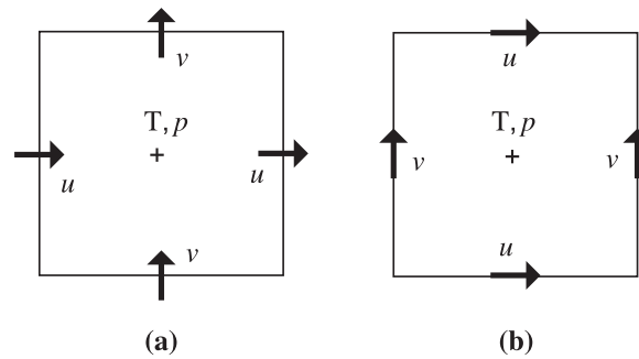
FIGURE 13.5 Horizontal grid staggering schemes for the Arakawa-C (a) and Arakawa-D (b) grids. Thermodynamic ( T, p ) and other scalar fields are located at the center of the grid cell; horizontal velocity components u and v are located along the grid edge.
