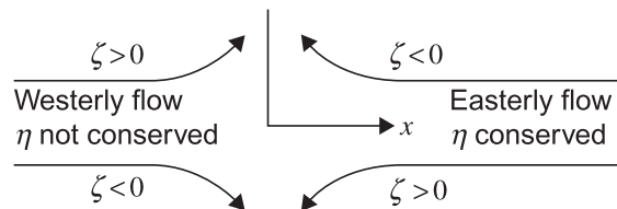
FIGURE 4.13 Absolute vorticity conservation for curved flow trajectories.
