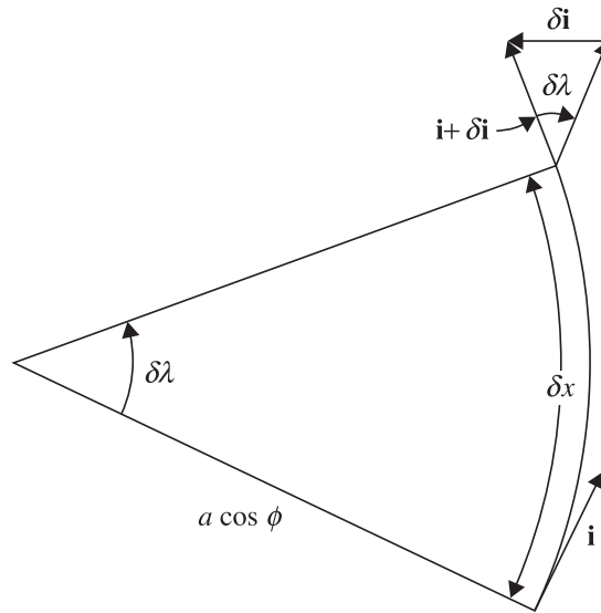
FIGURE 2.1 Longitudinal dependence of the unit vector \mathbf{i} .
