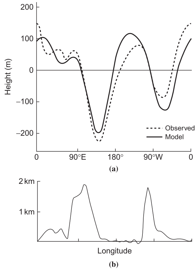
FIGURE 5.15 (a) Longitudinal variation of the disturbance in geopotential height ( \equiv f_0\Psi/g ) in the Charney–Eliassen model for the parameters given in the text ( solid line ) compared with the observed 500-hPa height perturbations at 45°N in January ( dashed line ). (b) Smoothed profile of topography at 45°N used in the computation. (After Held, 1983.)
